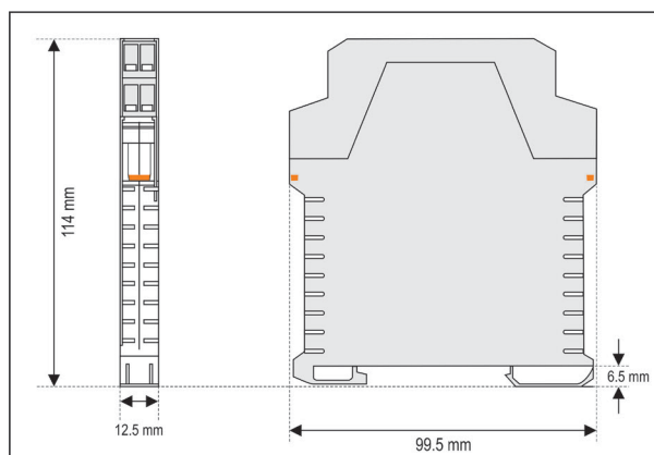
Fig. 4 – Transmitter dimensions
