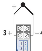
Fig. 9 – Transmitter electrical connections (Thermocouple)
