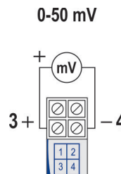
Fig. 10 – Transmitter electrical connections (0-50 mV)
