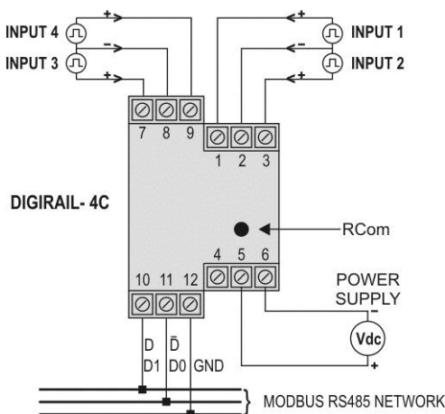
Figure 2 – Electrical Connections
