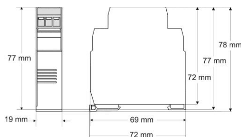
Figure 1 – Dimensions
