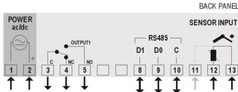
Figure 1 – N321 terminals
